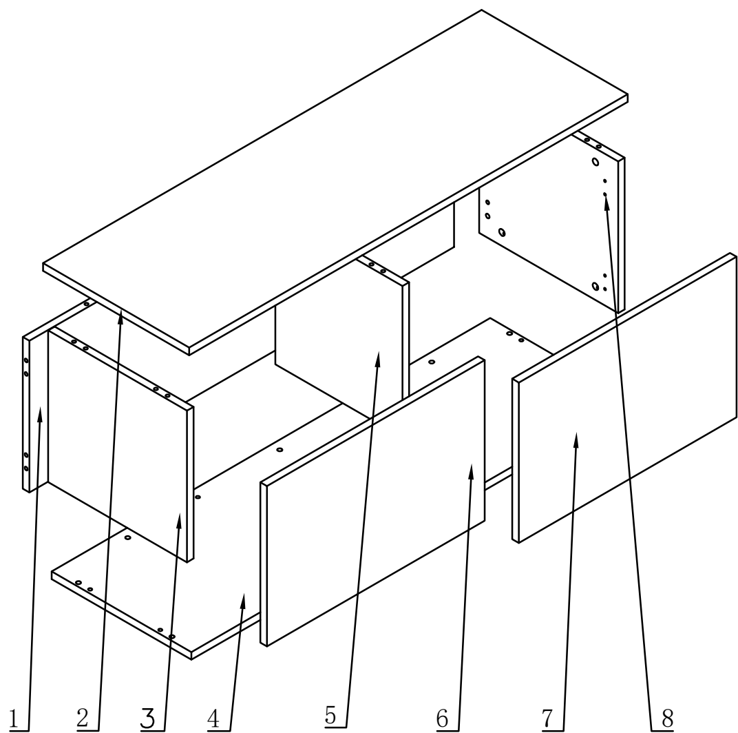
Exploded Diagram
